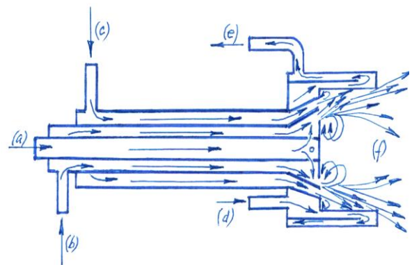
Figure 1. Constructive and functional scheme of the oxy-biofuel burner a – glycerol + ethanol; b – spraying water; c – oxygen; d – cooling water inlet; e – cooling water outlet; f – oxy-biofuel flame.
